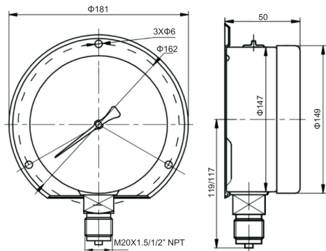
6" (150mm) Bottom Connection with optional Back Flange
