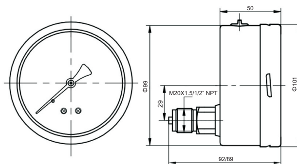
4" (100mm) Lower Back Connection
