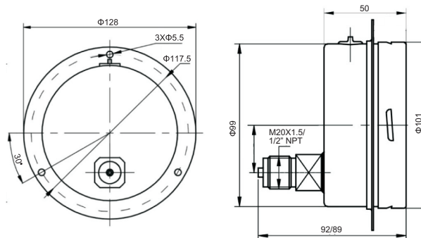
4" (100mm) Lower Back Connection with optional Front Flange
