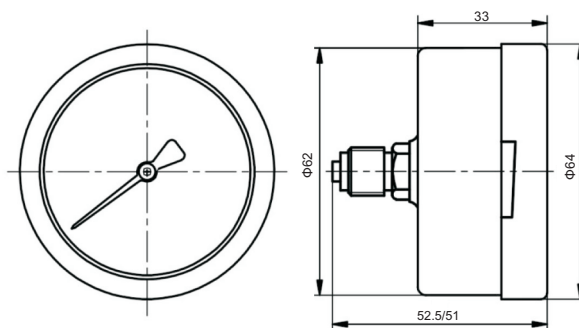
2.5" (63mm) Centre Back Connection
