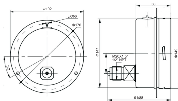
6" (150mm) Lower Back Connection with optional Front Flange
