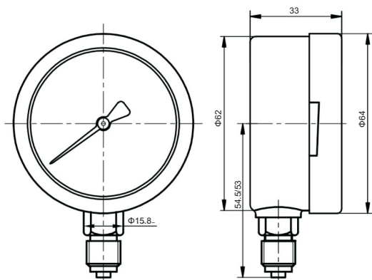
2.5" (63mm) Bottom Connection
