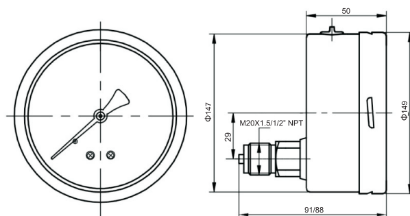
6" (150mm) Lower Back Connection
