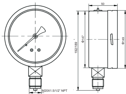
6" (150mm) Bottom Connection
