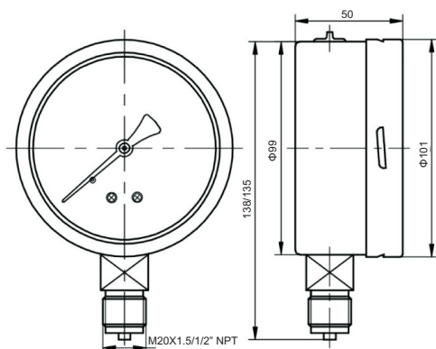
4" (100mm) Bottom Connection
