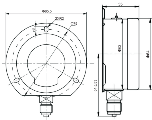
2.5" (63mm) Bottom Connection with optional Back Flange
