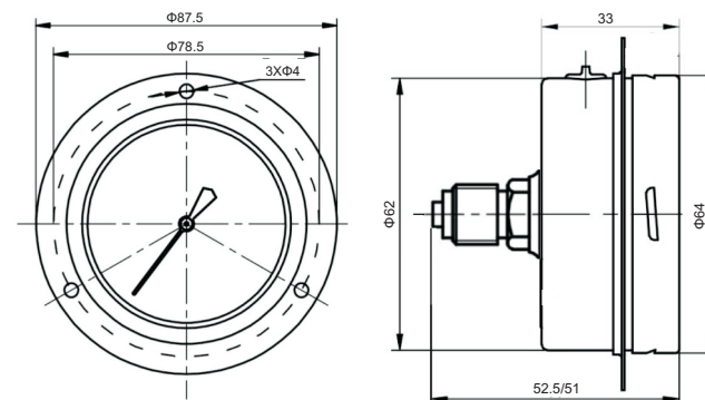
2.5" (63mm) Centre Back Connection with optional Front Flange
