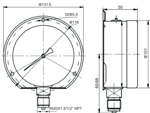
4" (100mm) Bottom Connection with optional Back Flange
